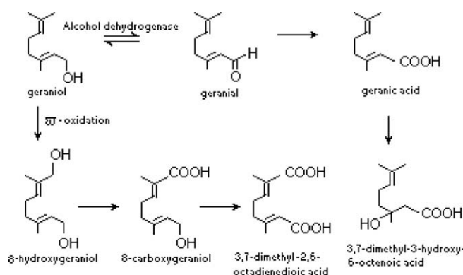
Fig. 1. Metabolism of geraniol in rats (Belsito et al., 2008).
